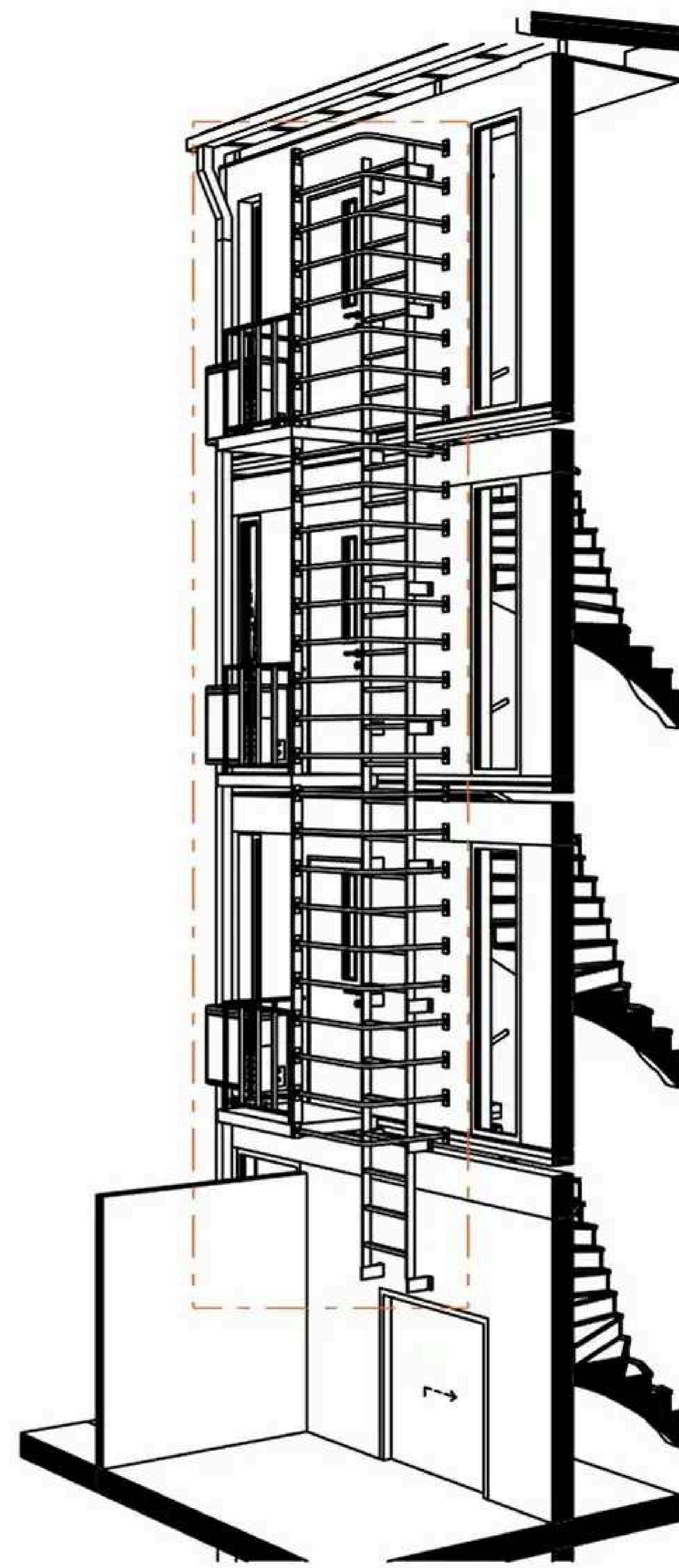
1:100 EGRESS 3D-01
