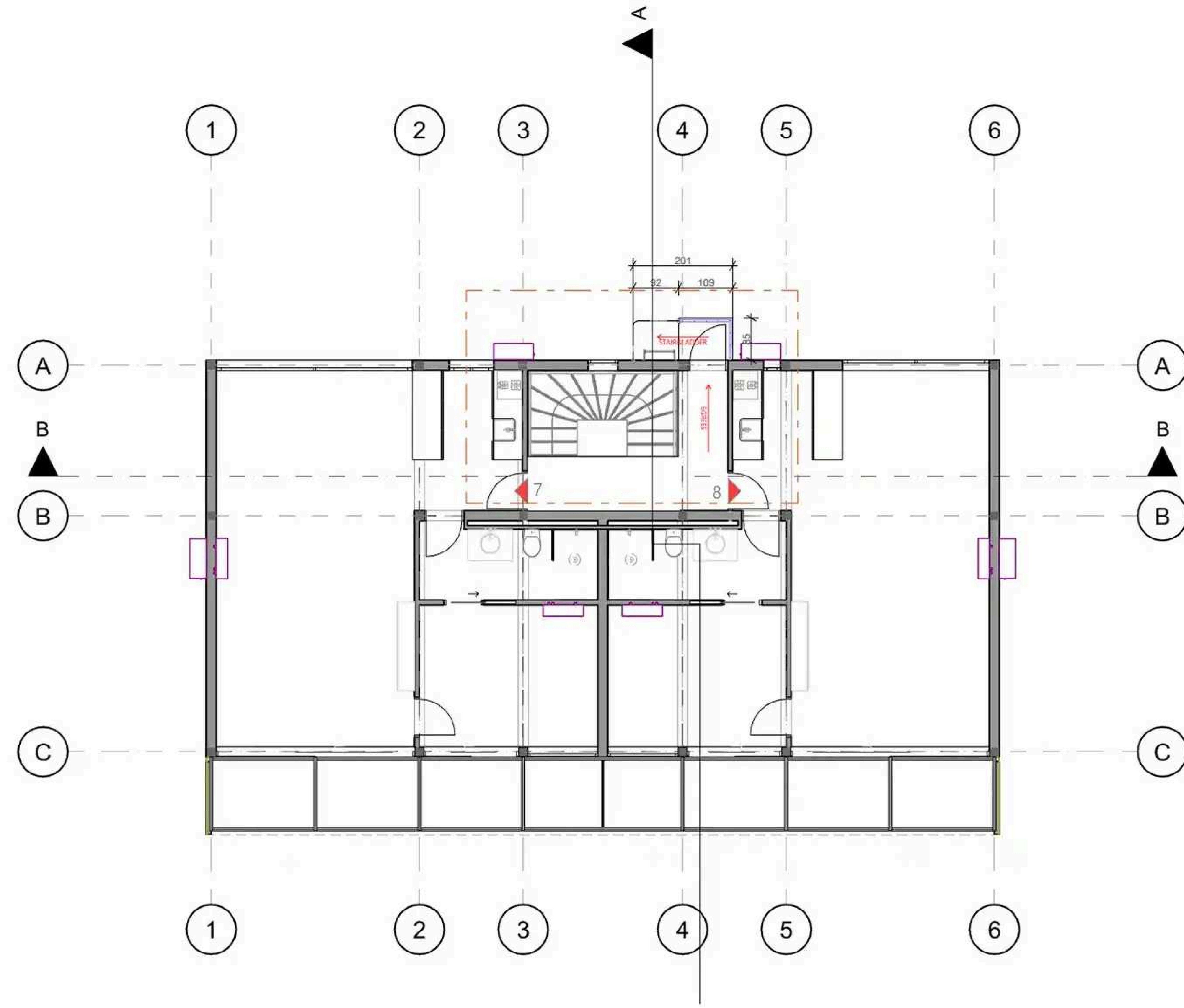
1:100 Story 3.
